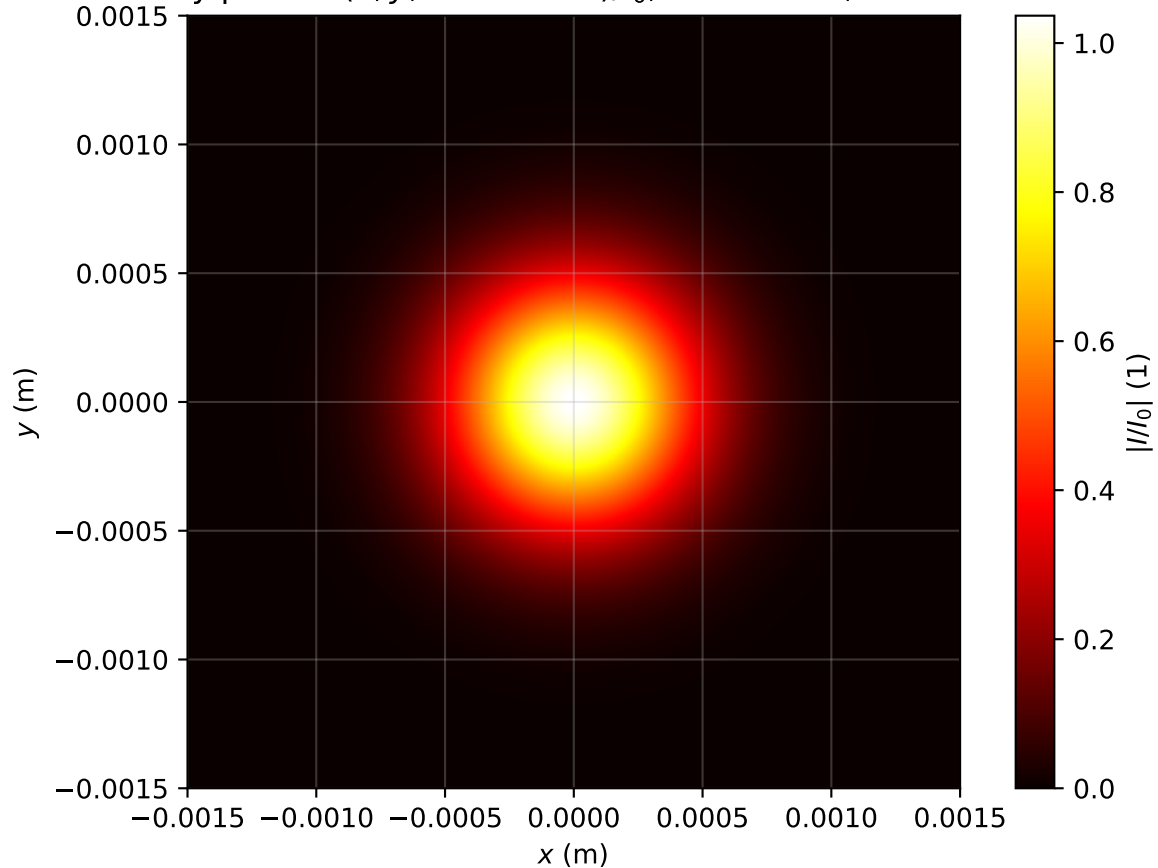
Intensity profile I(x, y, z = 0.239m)/I_0 , Pin=0.9Pcr, artificial time
